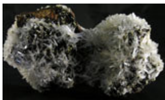
Hemimorphite & Mimeticite , Ojuela Mine, Mapimi, Durango, Mexico.
