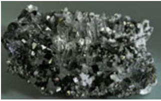
Pyrite, quartz and dolomite , Animon Mine, Pasco, Peru.
